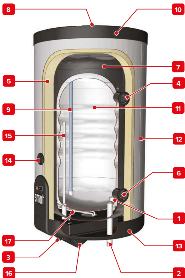
SLEW 100 - 130 - 160 - 210 - 240
